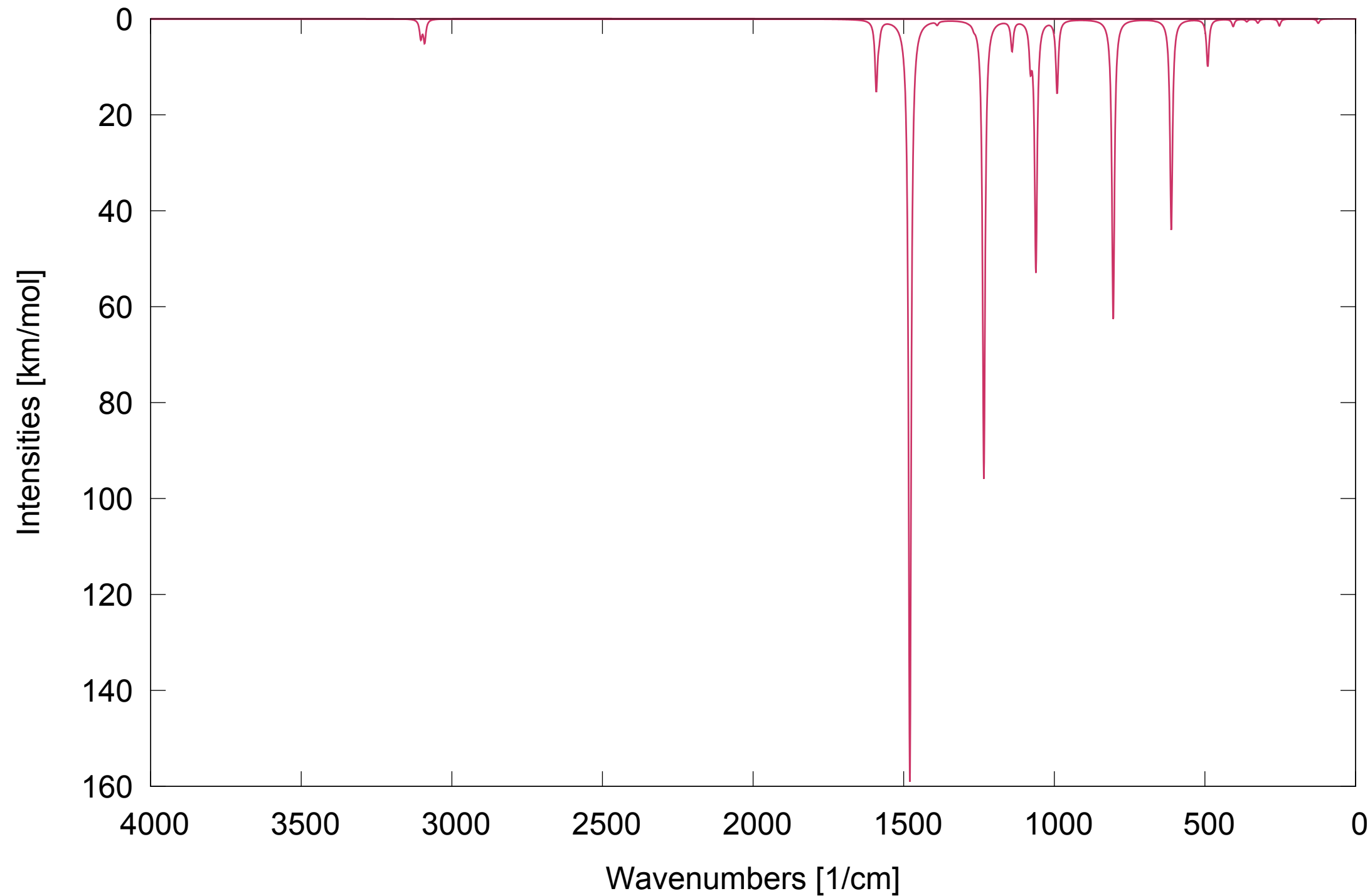
IR spectrum of CAS:352-33-0 level: B3LYP/6-31G(d)
