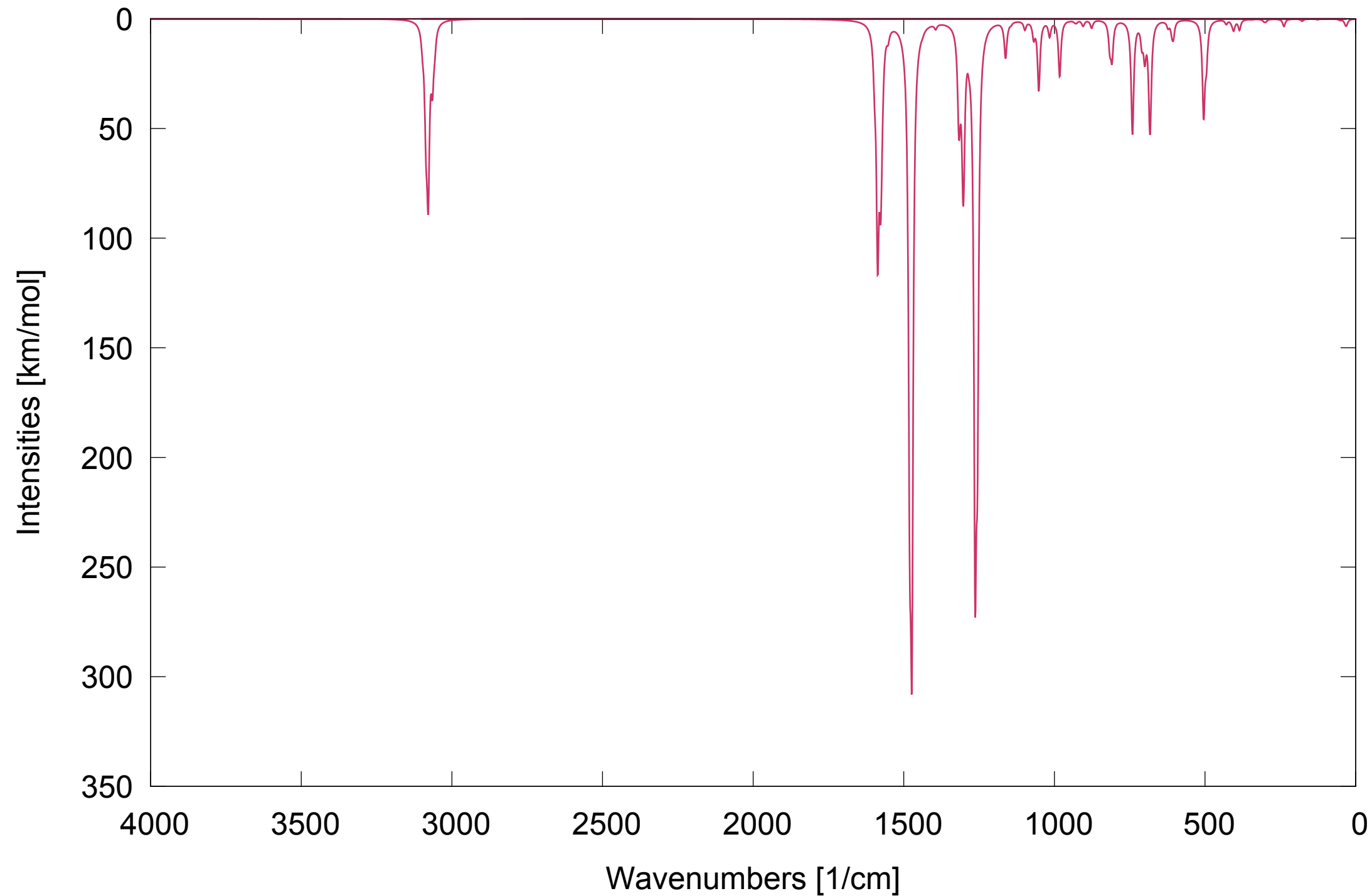
IR spectrum of CAS:36809-26-4 level: B3LYP/6-31G(d)
