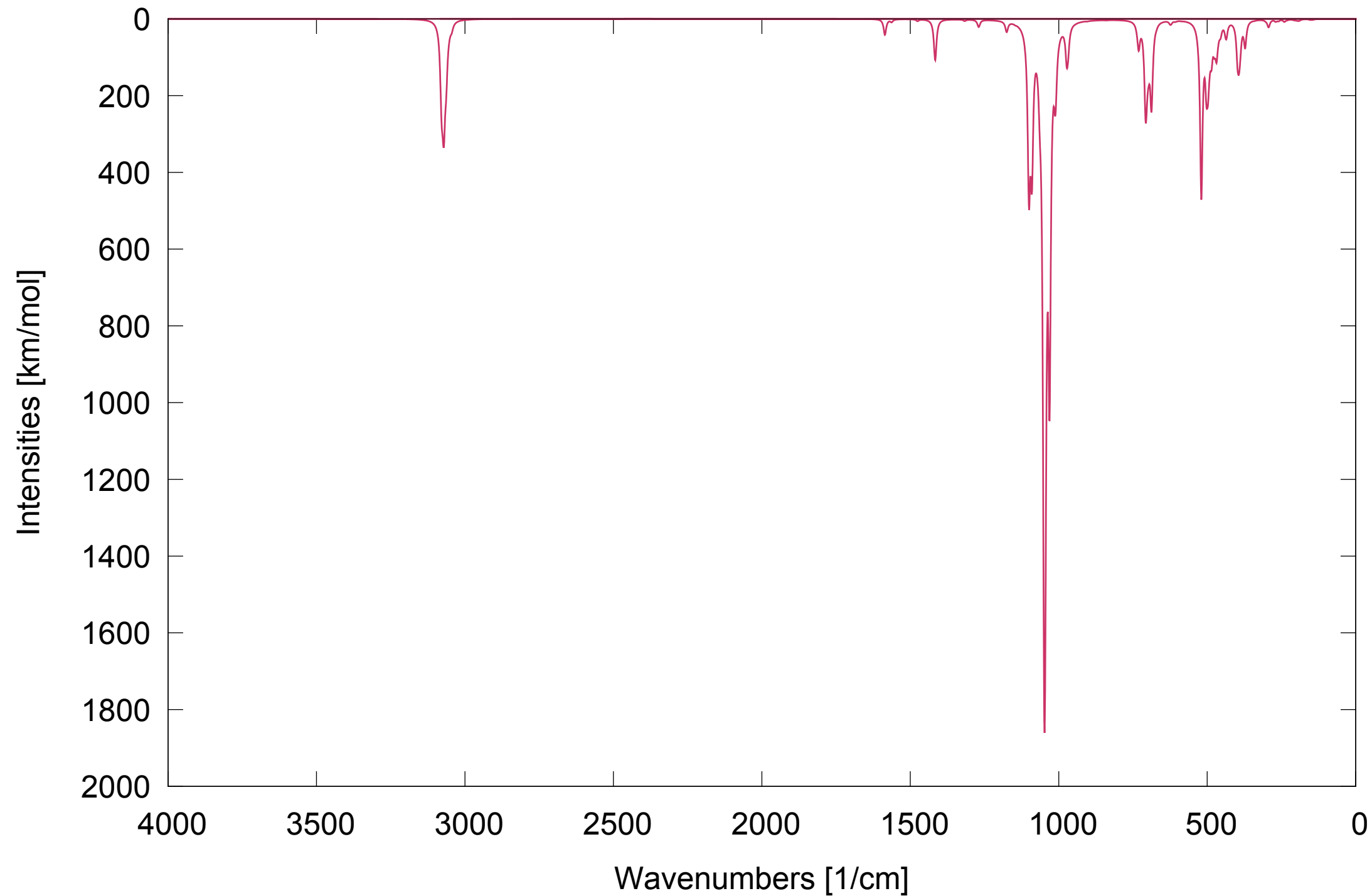
IR spectrum of CAS:546-56-5 level: B3LYP/6-31G(d)
