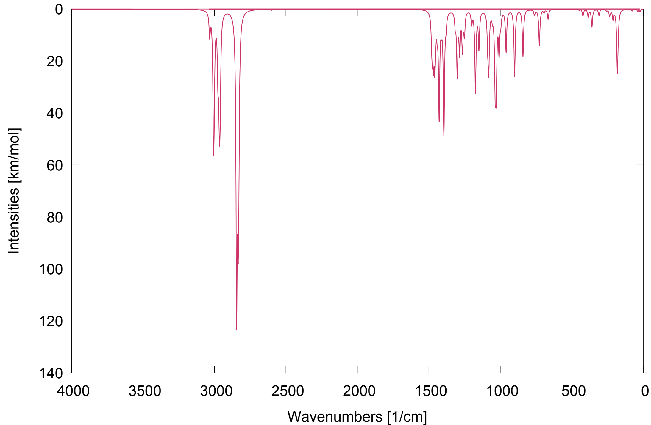
IR spectrum of CAS:61607-68-9 level: B3LYP/6-31G(d)
