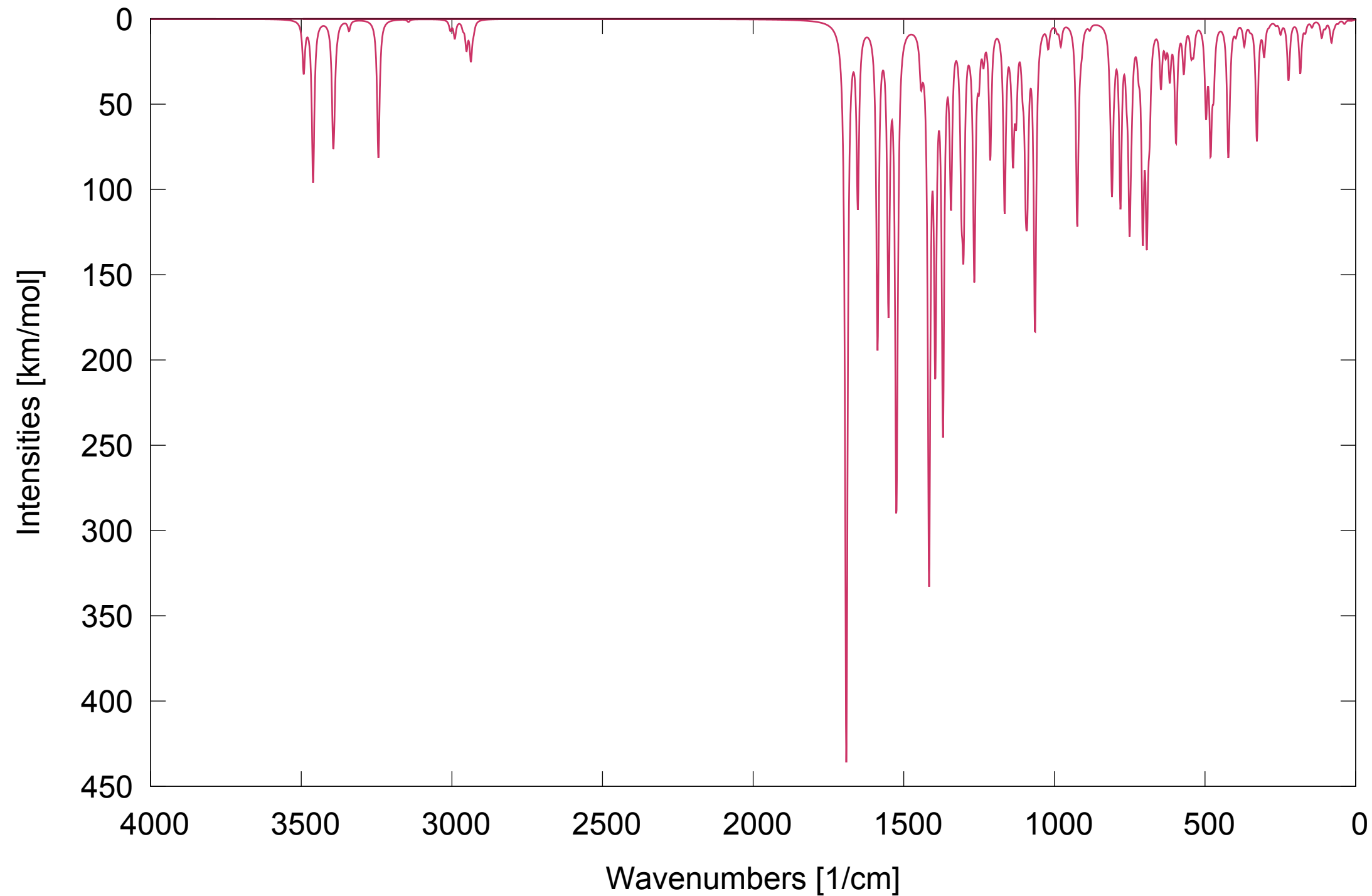
IR spectrum of CAS:76824-35-6 level: B3LYP/6-31G(d)
