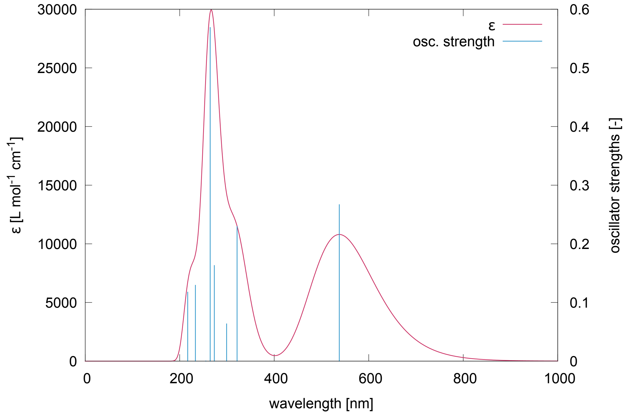
UV-VIS spectrum of compound at b3lyp/6-31g(d)
